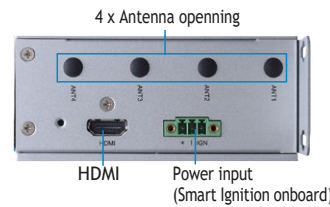
▲ Top view (Non-PoE SKU)
