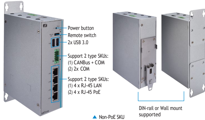
▲ Non-PoE SKU
